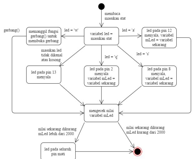
Gambar 12. Statechart fungsi LED(led)
