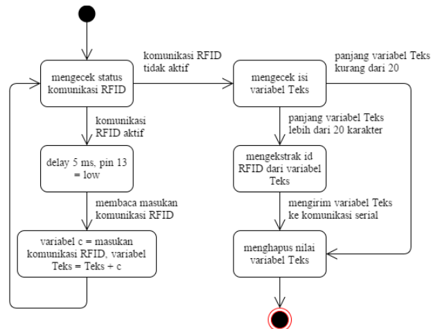
Gambar 11. Statechart fungsi cek()
