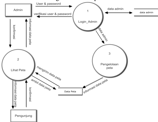
Gambar 3.5 DFD level 1
