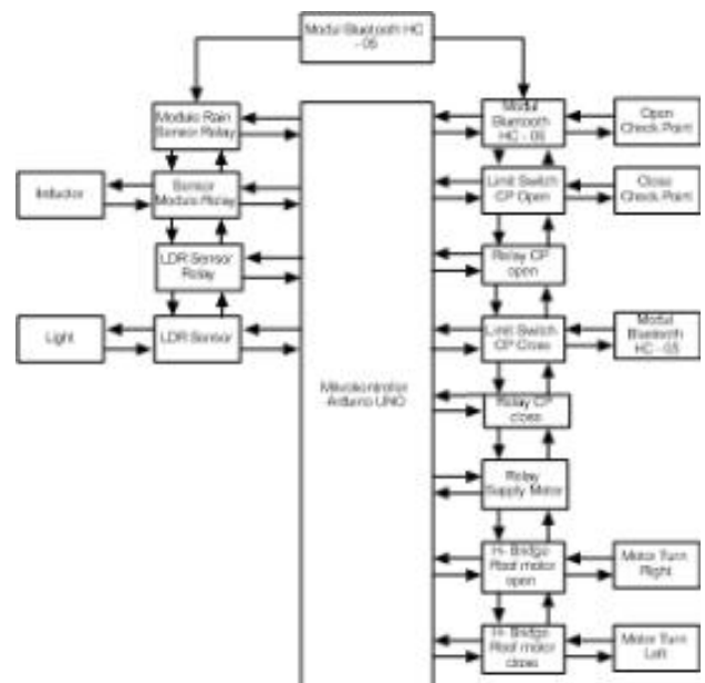
Gambar 2. Blok diagram
